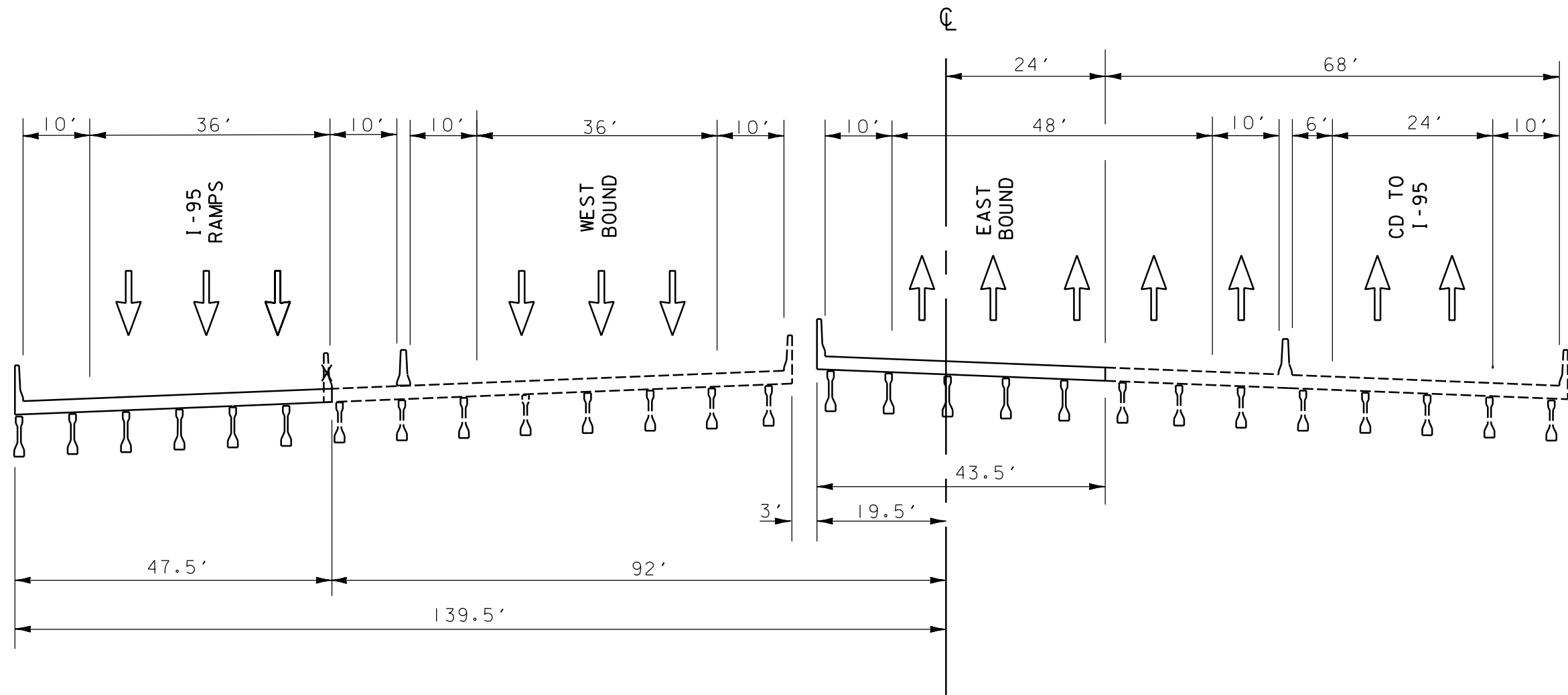
VIADUCT TYPICAL SECTION EAST OF SR 7 TO WEST OF I-95
